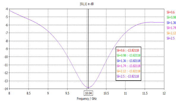
Figure 6: Graph return loss (S11) and resonant frequency from varying parameter.
