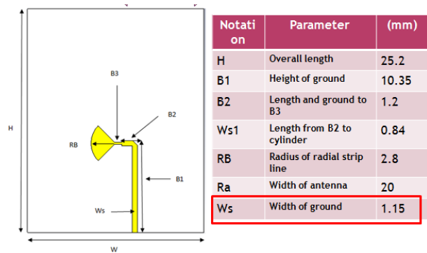
Figure 12: Back view of antenna with new value from parametric sweep.
