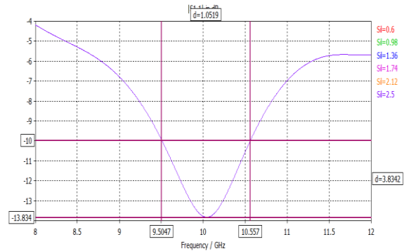
Figure 7: Graph return loss (S11) and bandwidth from varying parameter
